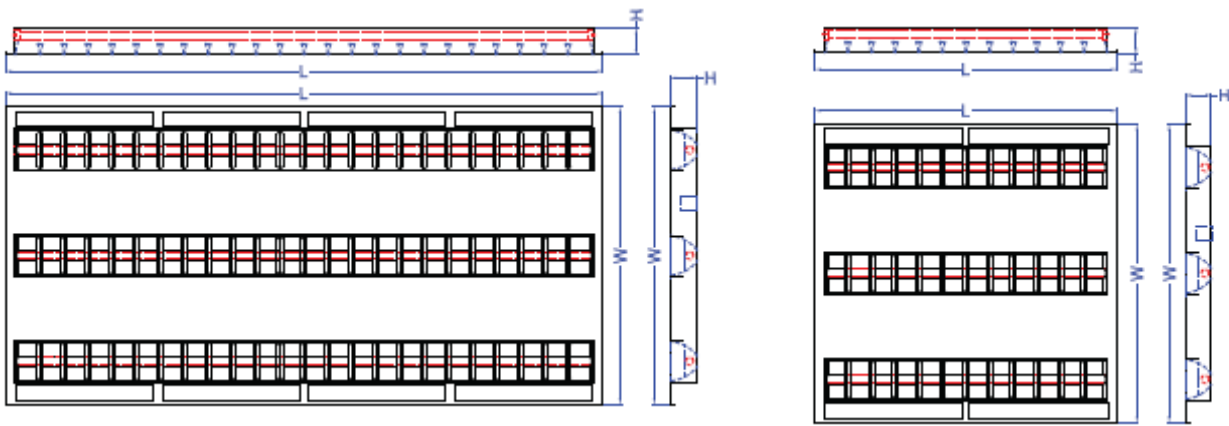
Lighting frame dimensions (燈具尺寸示意圖)
