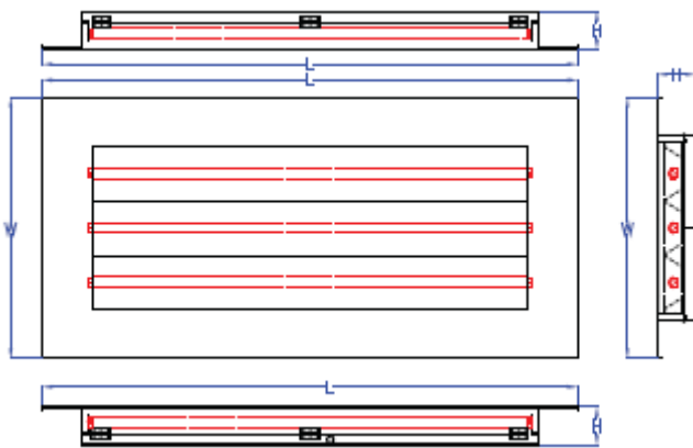
Lighting frame dimensions (燈具尺寸示意圖):
